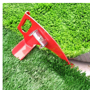
Seam Fix pressure tool for the solidified seaming process. Size(cm) 30x20x24 Weight (kg) 2.10
